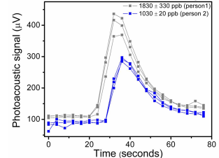
Fig. 5 Curves measured during thermodesorption, grey and blue squares indicate measurements of two volunteers. After gas sampling and baseline measurement the preconcentration unit is heated, therefore, ammonia releases. Ammonia concentrations are calculated from the area under the curves, mean concentration and standard deviation of the three consecutive measurements are indicated.
