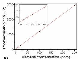
Fig. 2 Calibration curves of the instruments. Error bars show the standard deviation of data.
